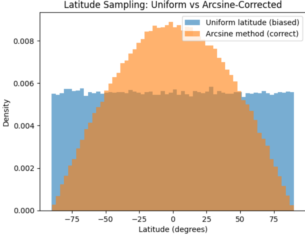
Figure 2: Comparison of uniform angular latitude sampling and spherical equal-area latitude sampling.
